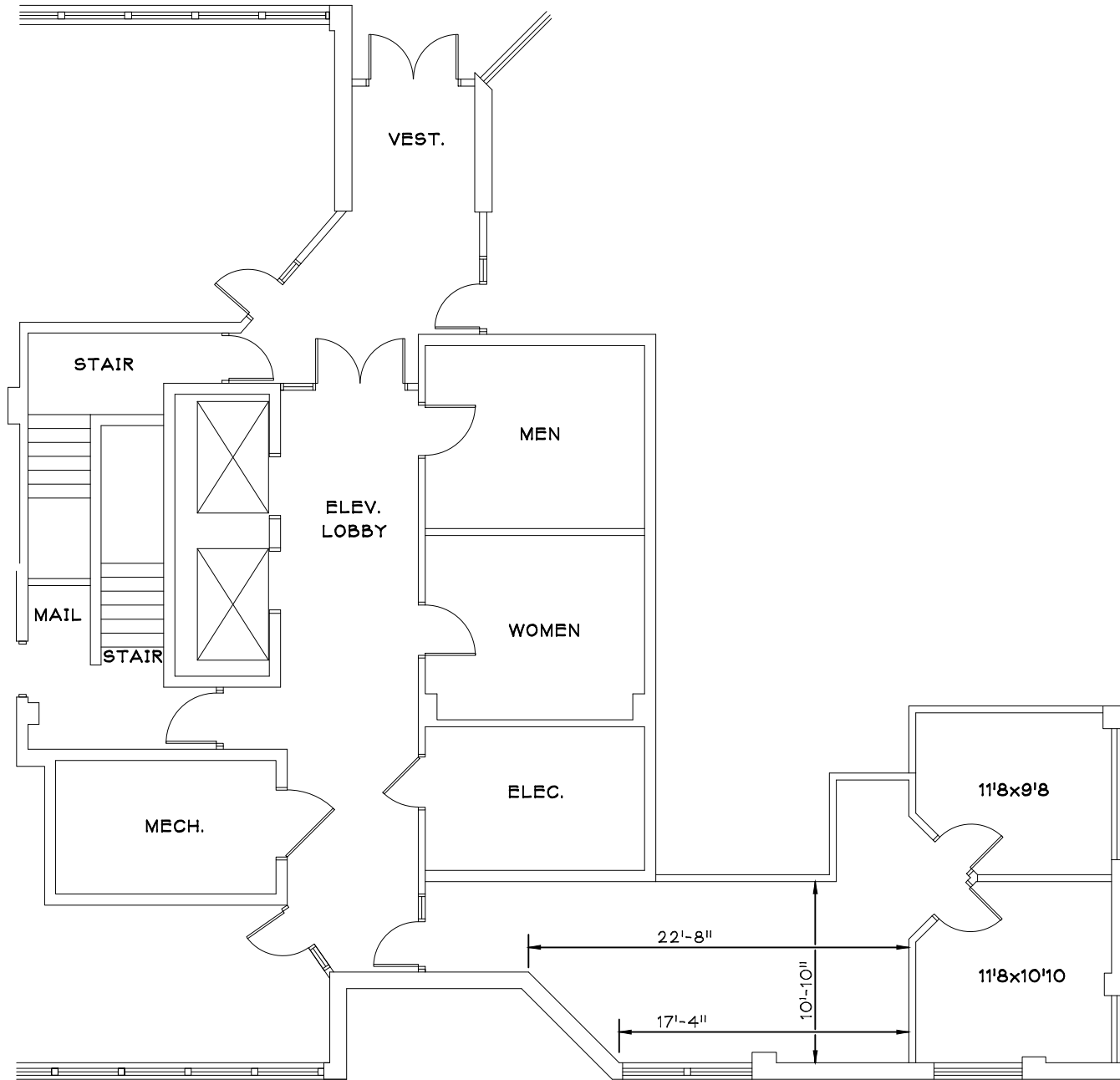
SOUTHMARK BUILDING FIRST FLOOR - SUITE 104 AS-BUILT PLAN
