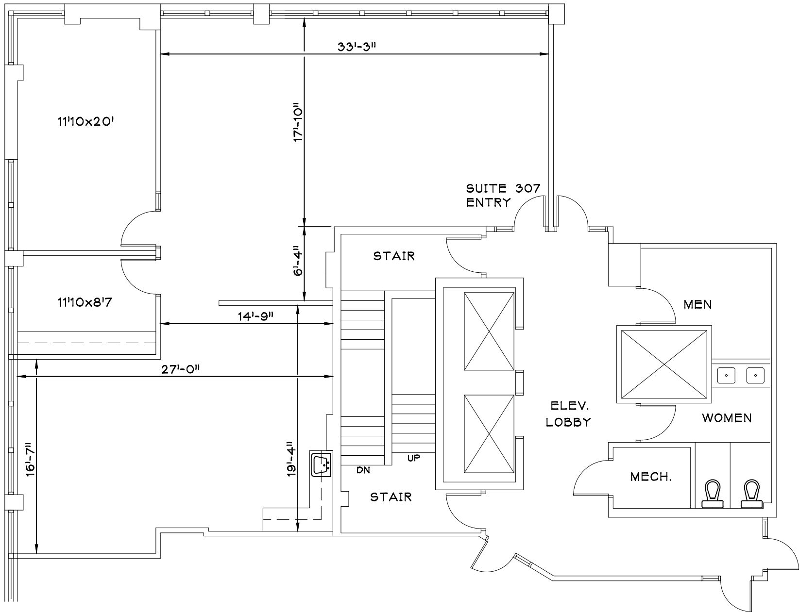
SOUTHMARK BUILDING THIRD FLOOR - SUITE 307 AS-BUILT PLAN
