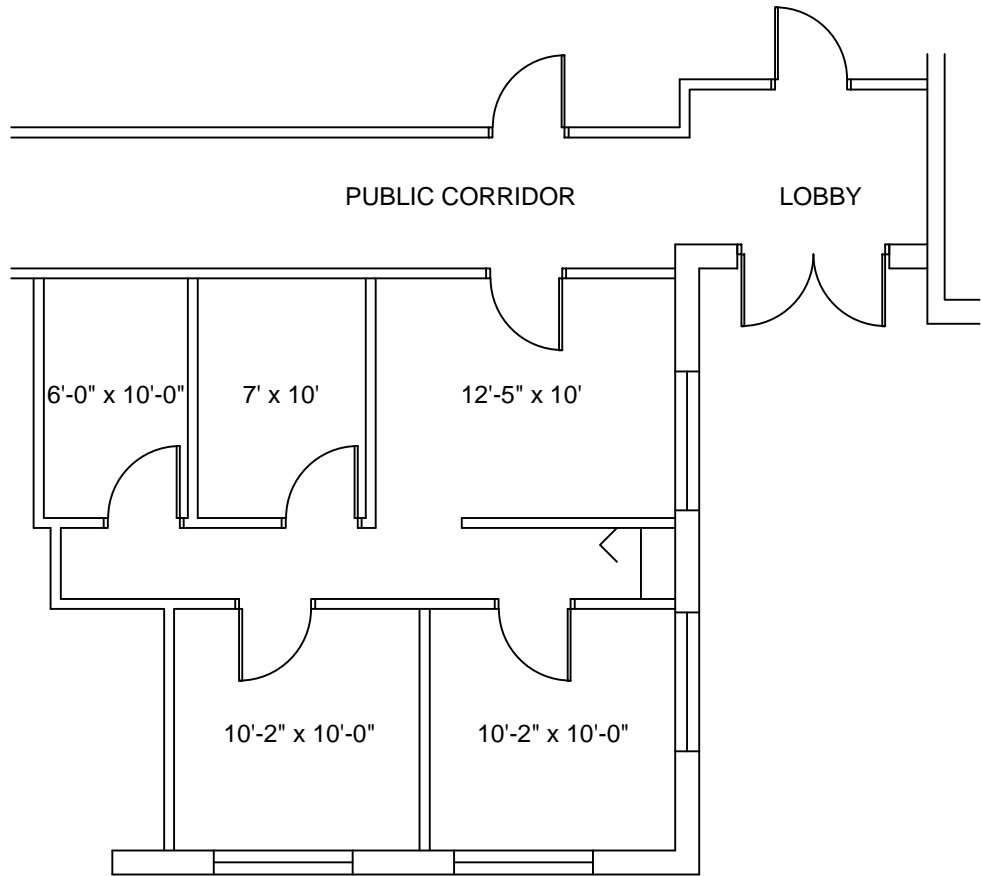
VILLAGE GREEN 850 BOYCE ROAD SUITE 6 AS-BUILT PLAN
